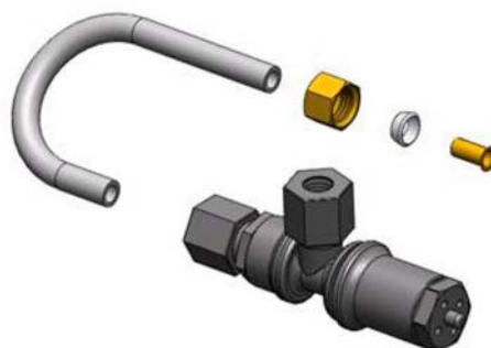
Valvola Salamoia 1600
